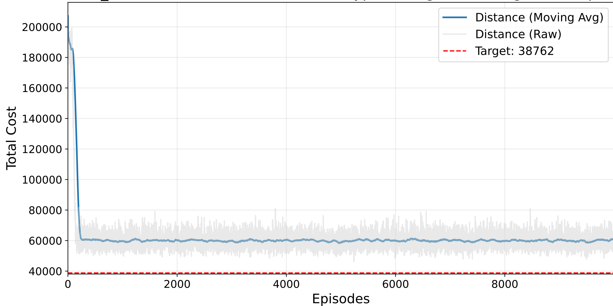
Final NO_BAYESIAN Masked AutoRL-SOP (HyperTuningSK) Training - kro124p.1.sop
